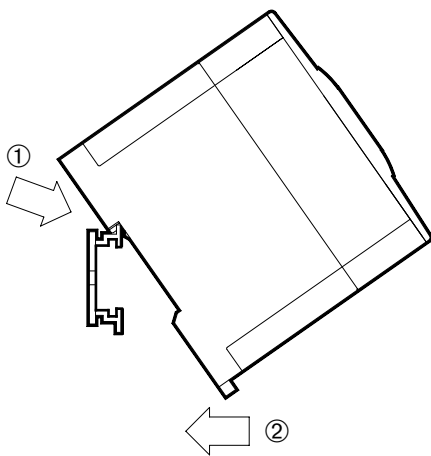
When attaching to DIN rail
